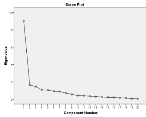
Figure 2: Scree Plot
